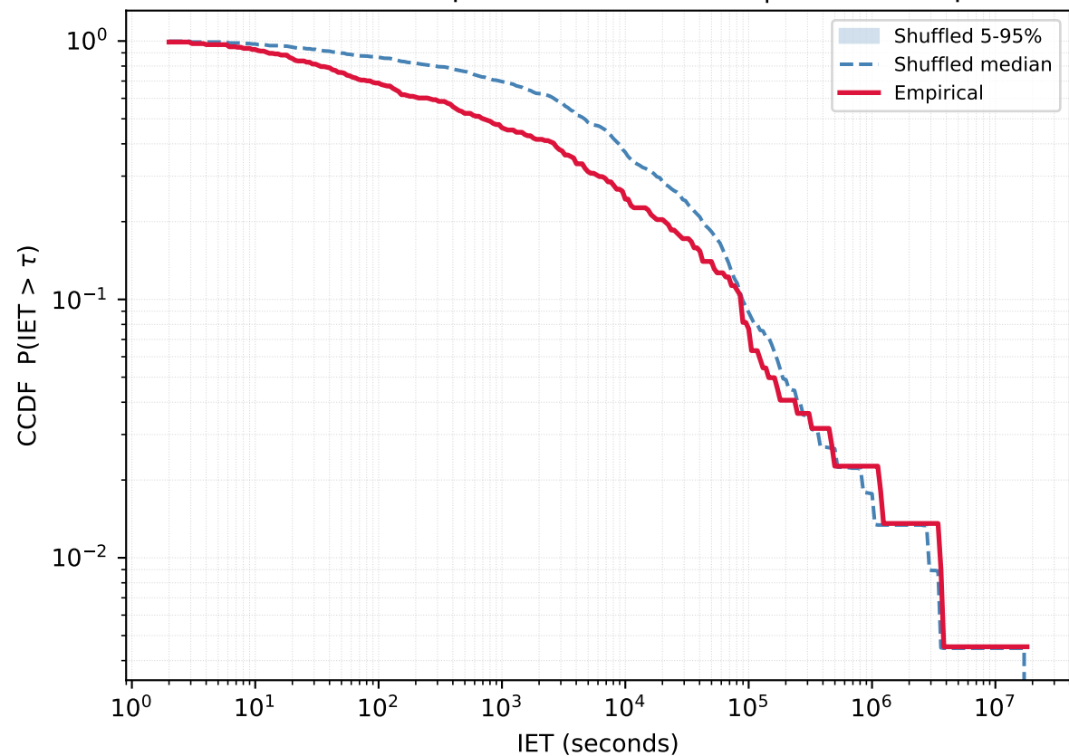
User 1110241832 - Empirical vs Reshuffled | KS=0.244 p=0.000
